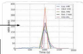
Figure 5: SRM131BB2 - CA TB 117 Urethane Foam
