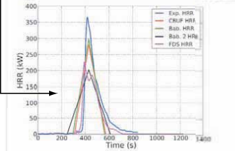
Figure 6: SRM111BS1 - Low density Urethane Foam
